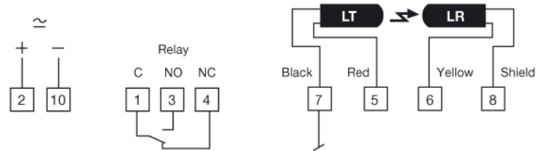
Relay output
