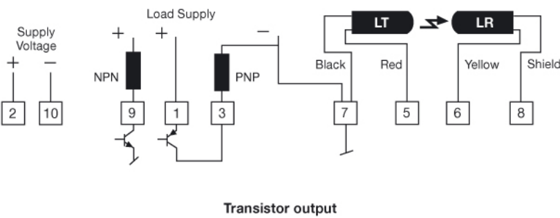
Transistor output
