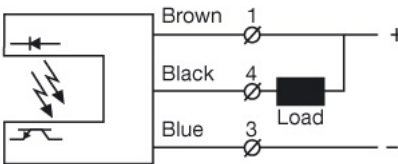
Load as NPN
