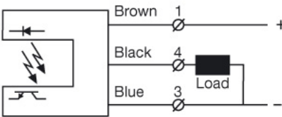
Load as PNP
